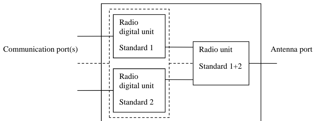
Figure 2: Multi-standard-radio equipment
